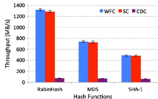
Fig. 2. Throughput of chunking and fingerprinting.
