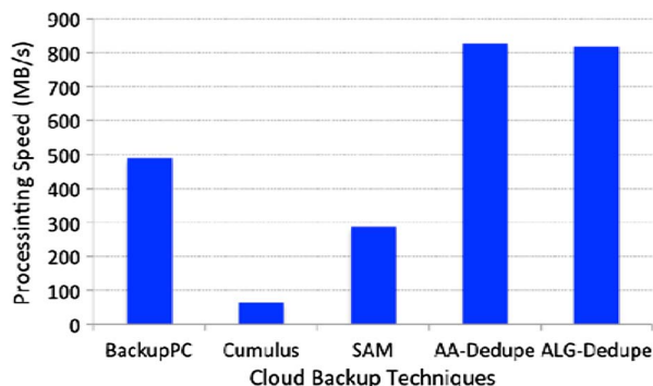
Fig. 11. Speeds of chunking and fingerprinting in PC clients.
