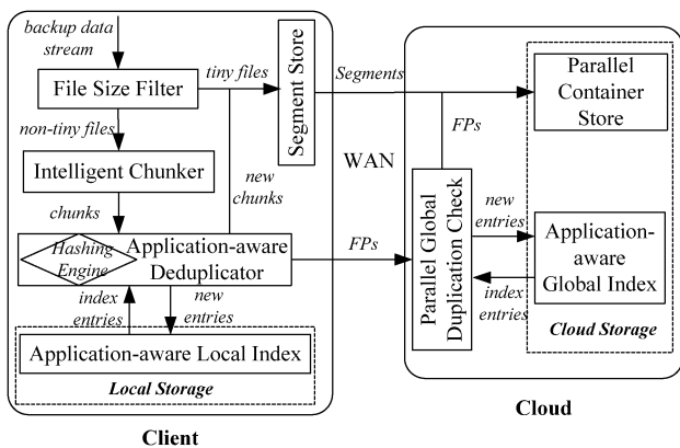
Fig. 4. Architectural overview of the ALG-Dedupe design.
