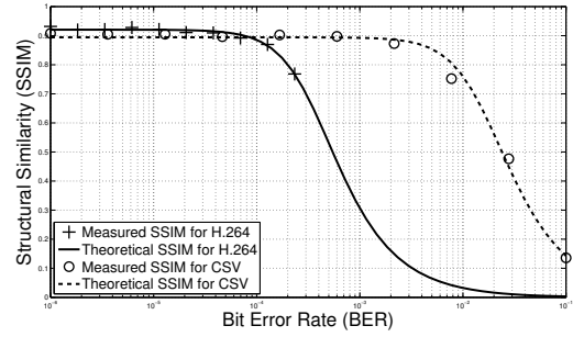
Fig. 18. SSIM of H.264 and CSV with channel errors.
