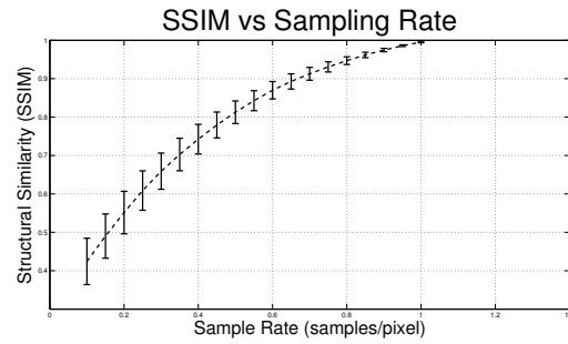
Fig. 4. Structural similarity (SSIM) index [22] for images with varying levels of sampling rate \gamma .
