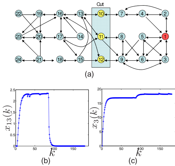
Fig. 7. (a) The network for the outdoor deployment. (b)-(c) The states of nodes 13 and 3, which are disconnected from and connected to, respectively, the source after the cut has occurred.
