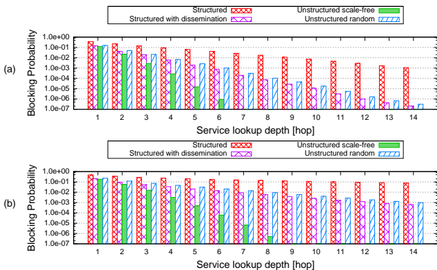
Fig. 2. Average blocking probability as a function of the service lookup depth D_l : comparison among structured, structured with epidemic dissemination, unstructured scale-free, and unstructured random overlays; (a) \rho_T = 0.6 ; (b) \rho_T = 0.9 .
