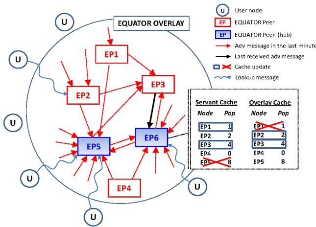
Fig. 4. EQUATOR architecture.
