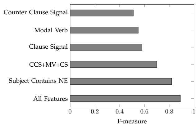
Fig. 2. Comparing the effectiveness of different features.
