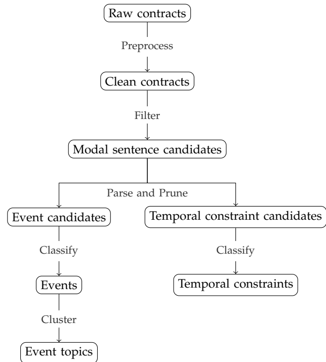
Fig. 1. Overall processing pipeline.
