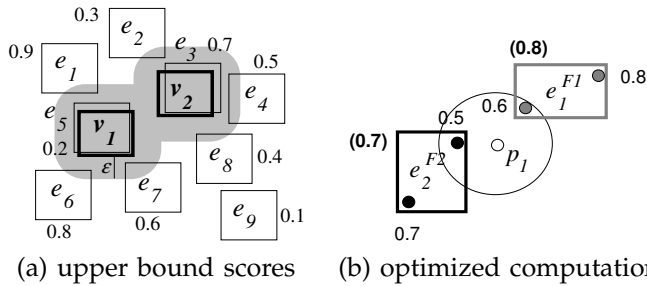
Fig. 4. Examples of deriving scores
