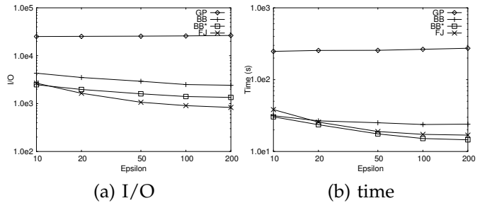
Fig. 16. Effect of \epsilon , influence scores
