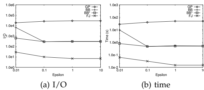
Fig. 17. Effect of \epsilon , range scores, real data
