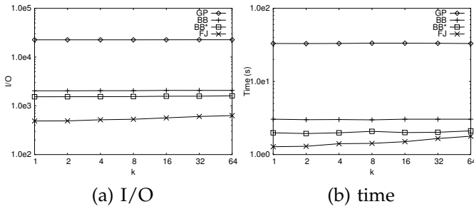
Fig. 12. Effect of k , range scores
